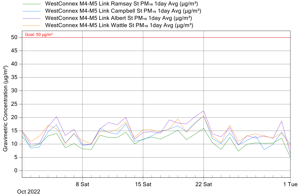
Figure 4: WCX M4-M5 Link Project Air Monitoring Stations - PM 10 24-Hour Averages Graph for October 2022
