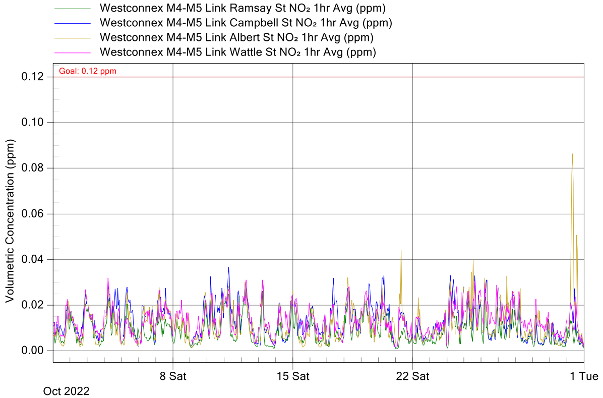
Figure 3: WCX M4-M5 Link Project Air Monitoring Stations - NO 2 1-Hour Averages Graph for October 2022
