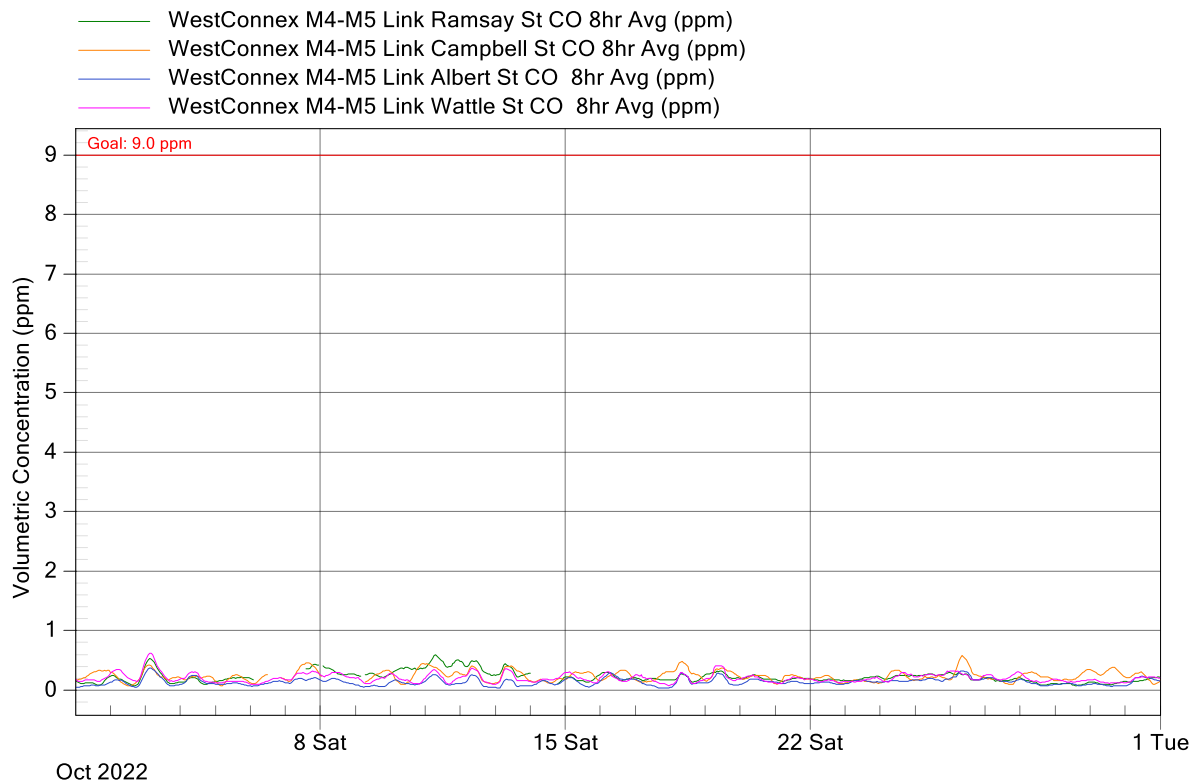
Figure 2: WCX M4-M5 Link Project Air Monitoring Stations - CO 8-Hour Rolling Graph for October 2022
