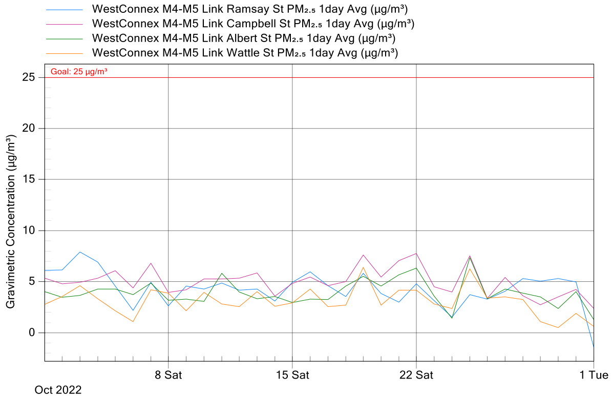
Figure 5: WCX M4-M5 Link Project Air Monitoring Stations - PM 2.5 24-Hour Averages Graph for October 2022
