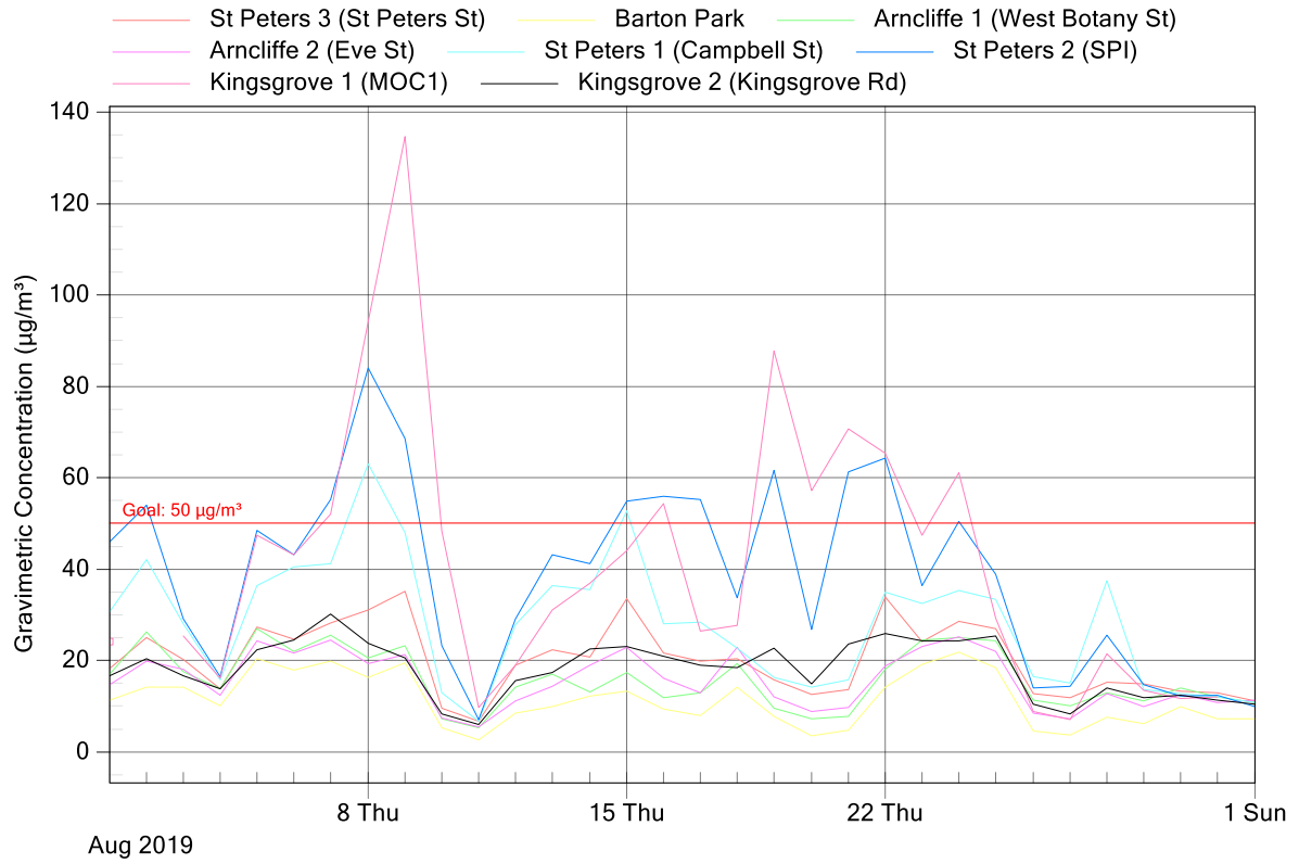
Figure 4: New M5 Project Air Monitoring Stations - PM 10 24 Hour graph for August 2019
