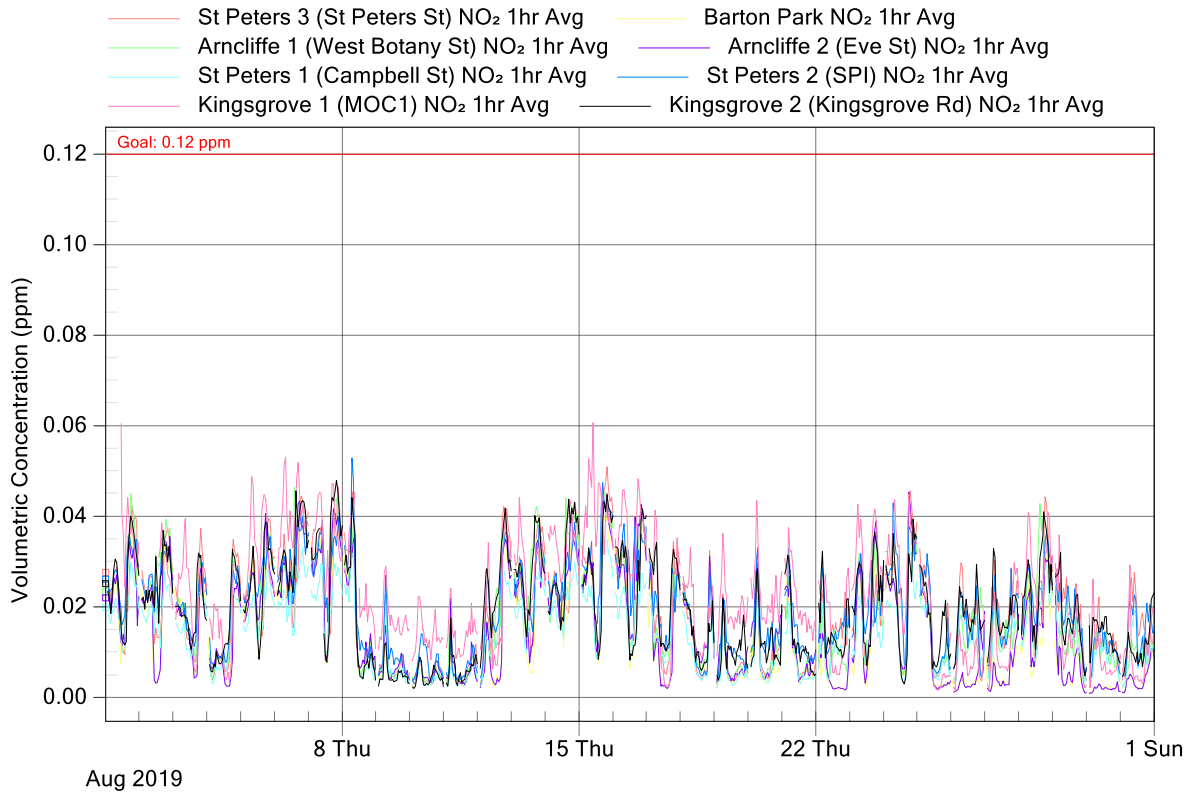
Figure 3: New M5 Project Air Monitoring Stations - NO 2 graph for August 2019
