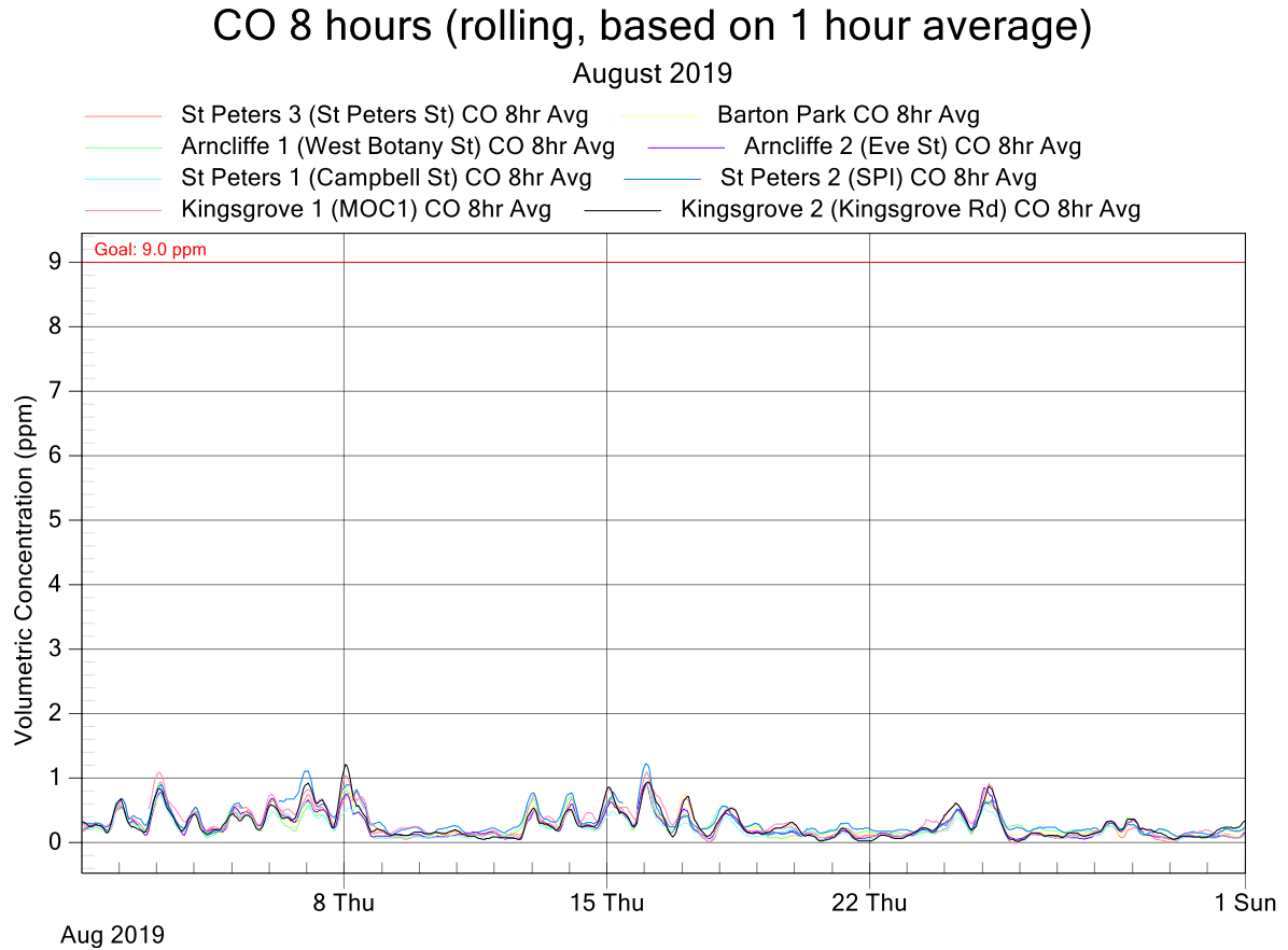
Figure 2: New M5 Project Air Monitoring Stations - CO 8 hours rolling graph for August 2019
