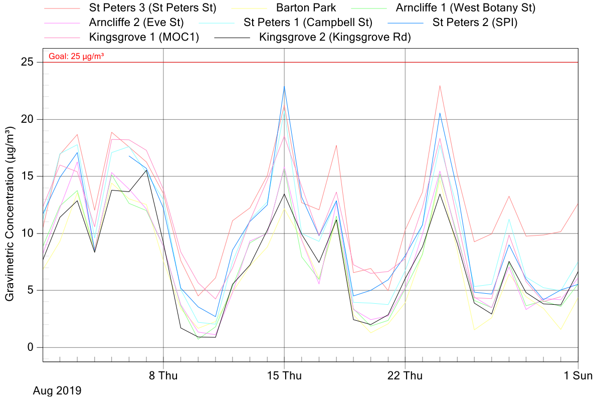
Figure 5: New M5 Project Air Monitoring Stations - PM 2.5 24 Hour graph August 2019
