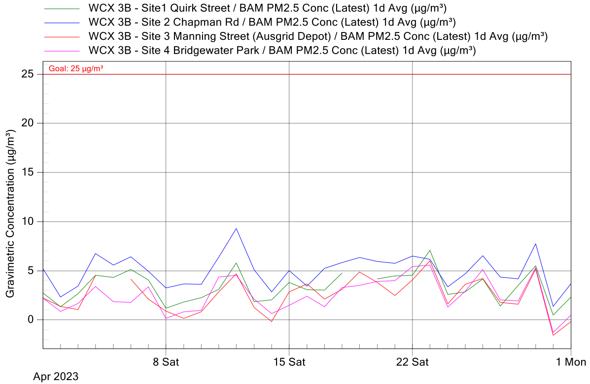
Figure 5: WCX 3B Project Air Monitoring Stations - PM 2.5 24-Hour Averages Graph for April 2023
