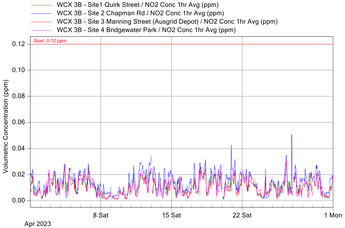
Figure 3: WCX 3B Project Air Monitoring Stations - NO 2 1-Hour Averages Graph for April 2023
