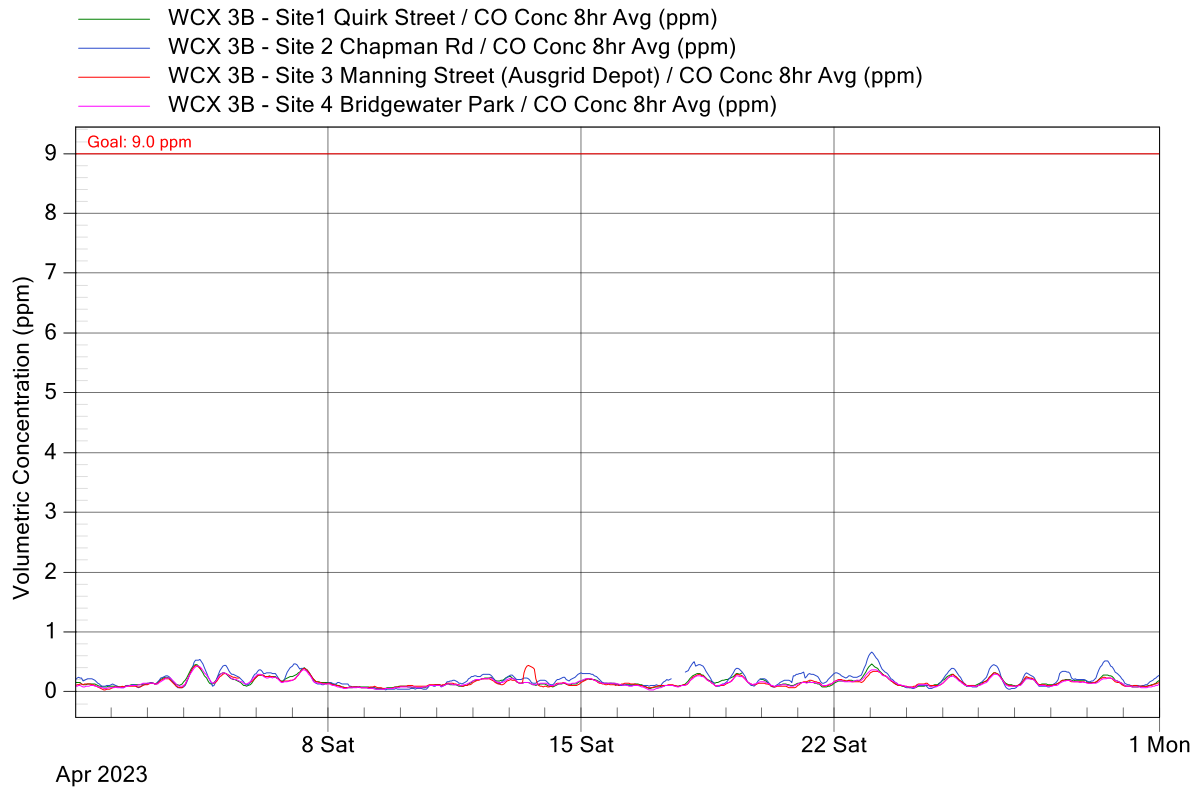
Figure 2: WCX 3B Project Air Monitoring Stations - CO 8-Hour Rolling Graph for April 2023
