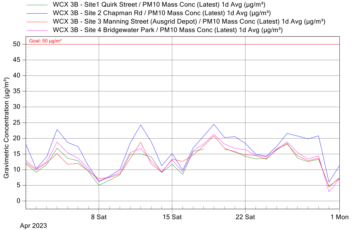
Figure 4: WCX 3B Project Air Monitoring Stations - PM 10 24-Hour Averages Graph for April 2023
