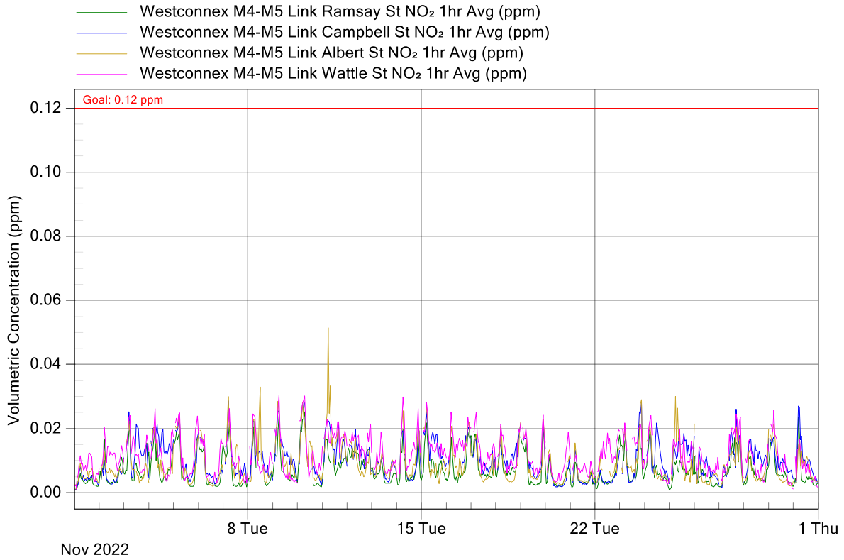
Figure 3: WCX M4-M5 Link Project Air Monitoring Stations - NO 2 1-Hour Averages Graph for November 2022
