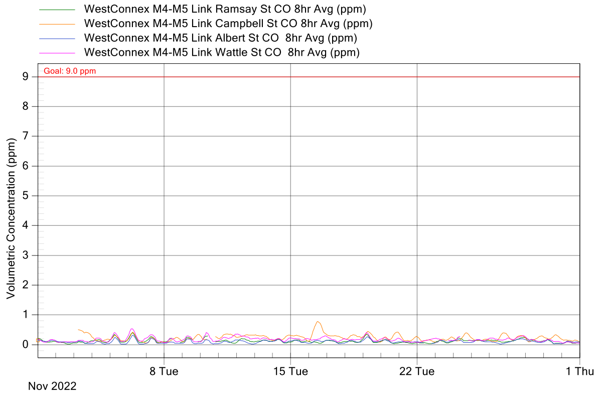
Figure 2: WCX M4-M5 Link Project Air Monitoring Stations - CO 8-Hour Rolling Graph for November 2022
