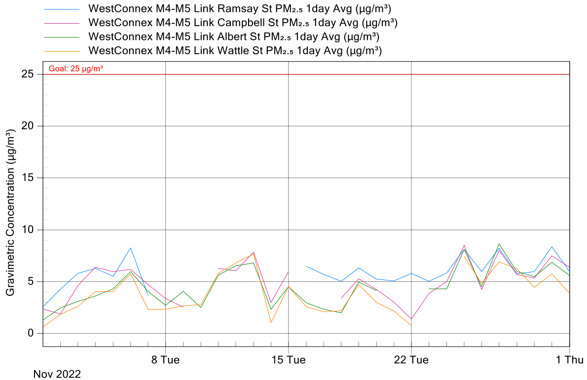
Figure 5: WCX M4-M5 Link Project Air Monitoring Stations - PM 2.5 24-Hour Averages Graph for November 2022
