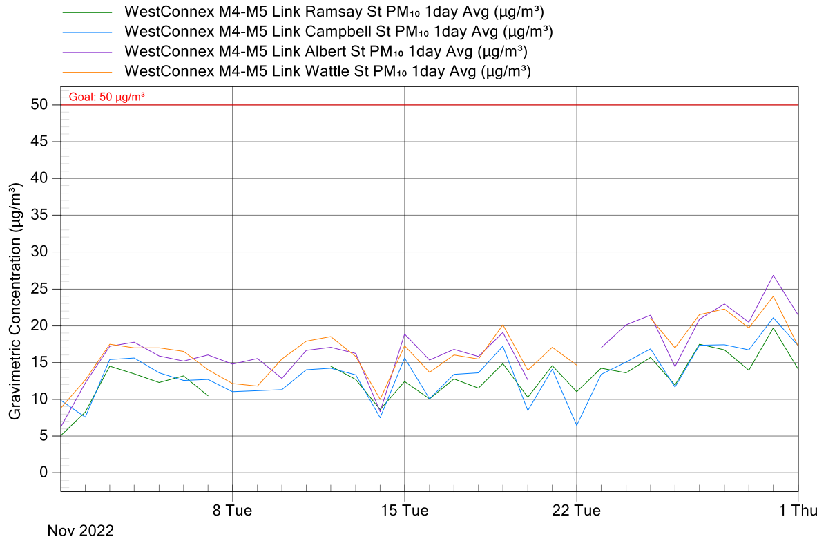
Figure 4: WCX M4-M5 Link Project Air Monitoring Stations - PM 10 24-Hour Averages Graph for November 2022
